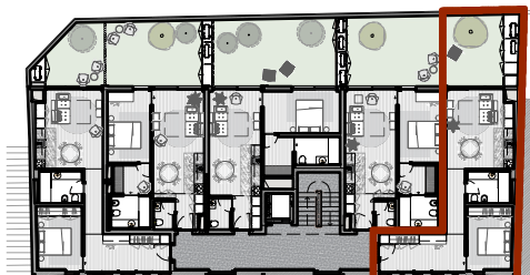
Floor-Plan
